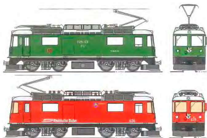
Type sketch and paint scheme sample Ge 4/4 II
